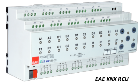
EAE KNX RCU ROOM CONTROL UNIT
